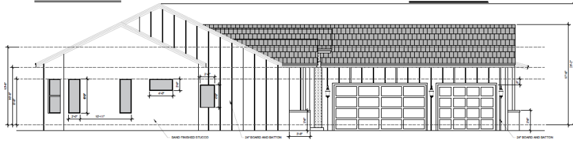
LEFT ELEVATION
