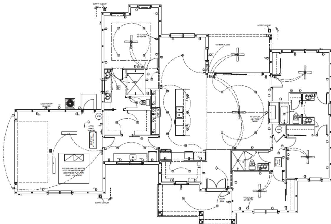
ELECTRICAL PLAN
