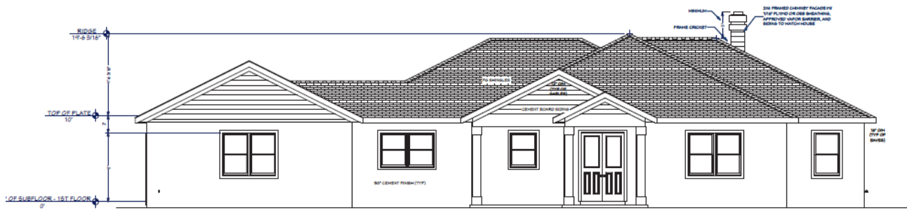
FRONT ELEVATION 1/4" = 1 FT
