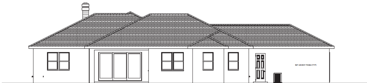
REAR ELEVATION 1/4" = 1 FT
