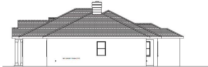
RIGHT ELEVATION 1/4" = 1 FT
