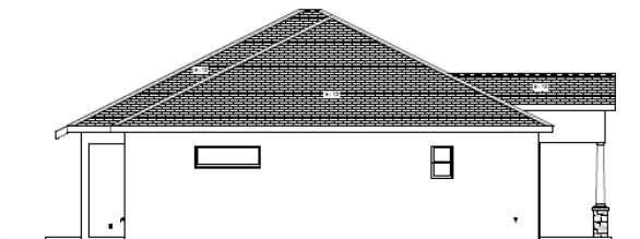
LEFT ELEVATION 1/4 IN = 1 FT
