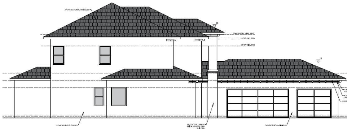
LEFT ELEVATION
